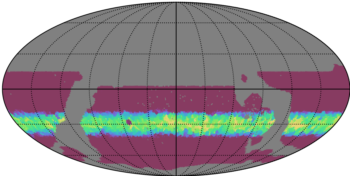
ddf_loaded_half_fl2_v3.4_10yrs WFD z band: Min normairmass
