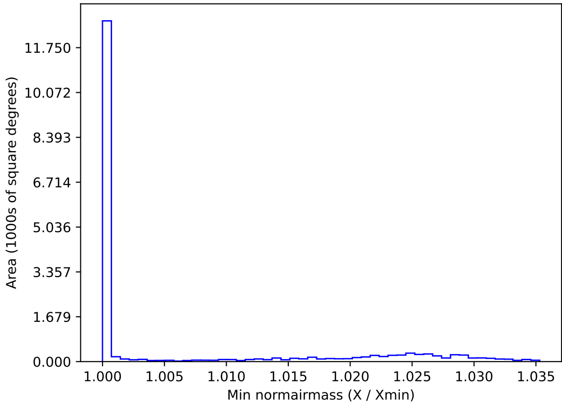
ddf_loaded_half_fl2_v3.4_10yrs WFD z band: Min normairmass
