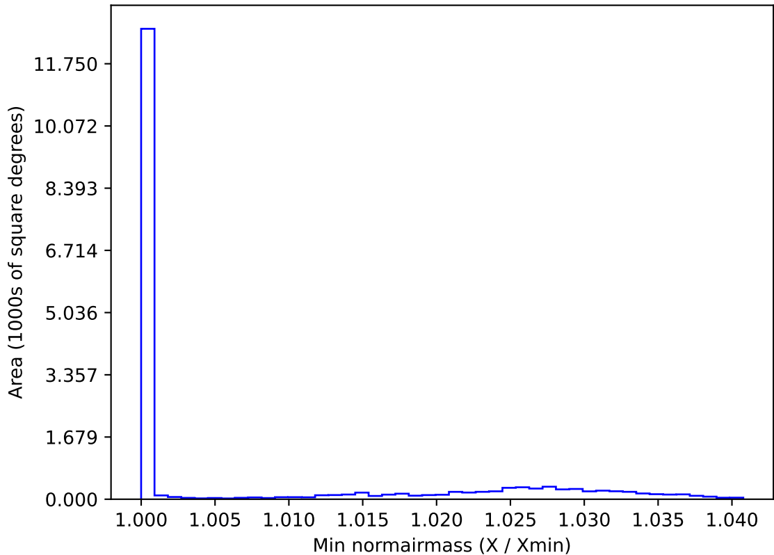
ddf_loaded_half_fl2_v3.4_10yrs WFD y band: Min normairmass
