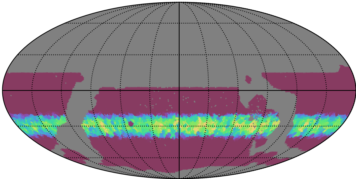
ddf_loaded_half_fl2_v3.4_10yrs WFD r band: Min normairmass
