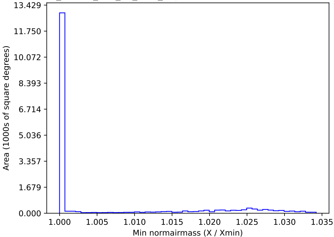
ddf_loaded_half_fl2_v3.4_10yrs WFD i band: Min normairmass
