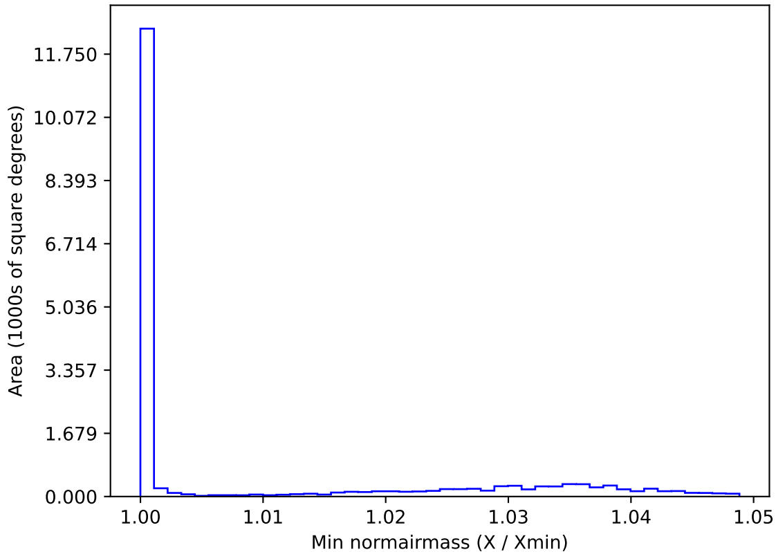
ddf_loaded_half_fl2_v3.4_10yrs WFD g band: Min normairmass
