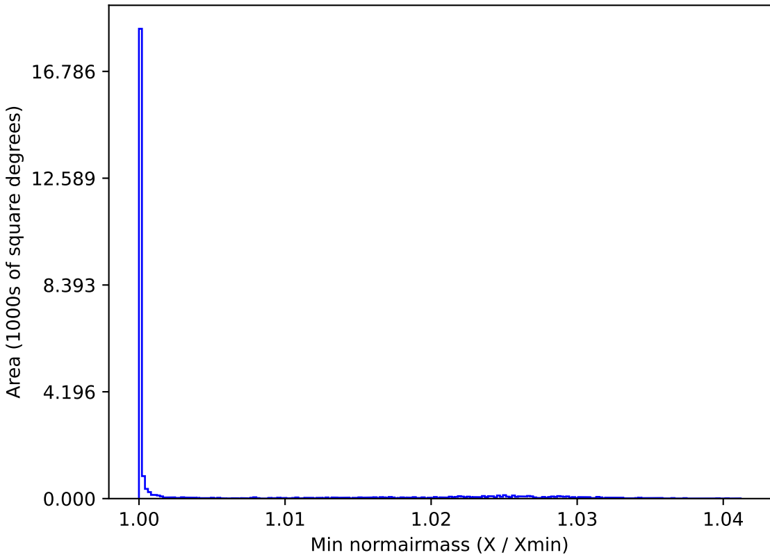
ddf_loaded_half_fl2_v3.4_10yrs All sky z band: Min normairmass
