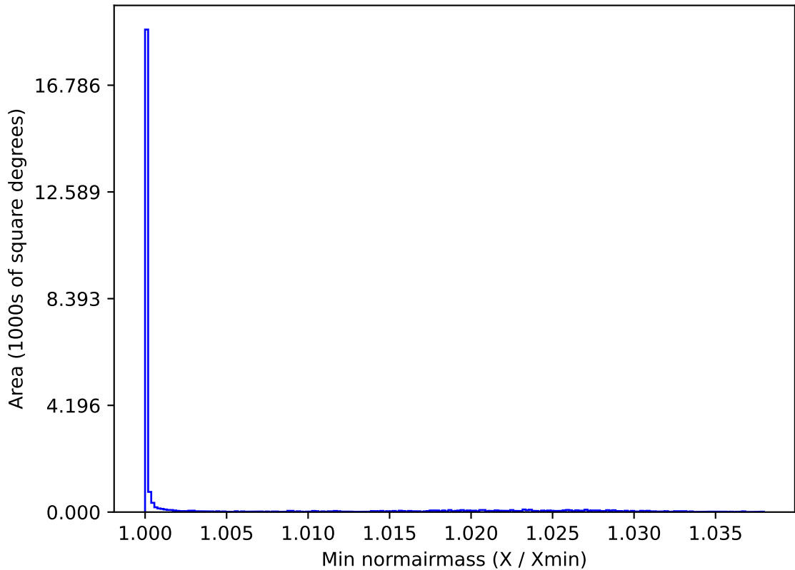
ddf_loaded_half_fl2_v3.4_10yrs All sky r band: Min normairmass
