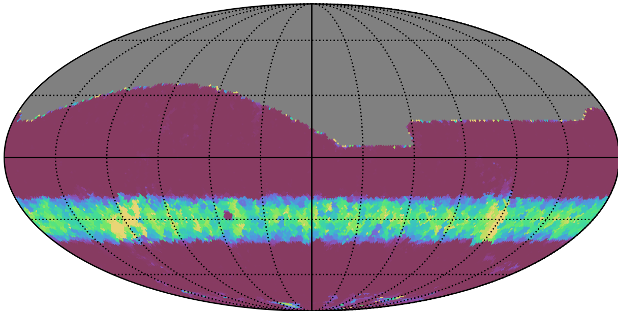
ddf_loaded_half_fl2_v3.4_10yrs All sky g band: Min normairmass
