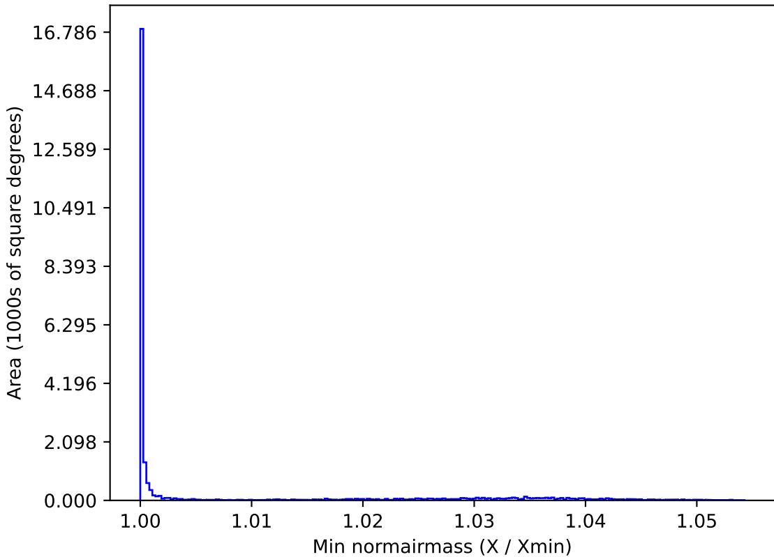
ddf_loaded_half_fl2_v3.4_10yrs All sky g band: Min normairmass
