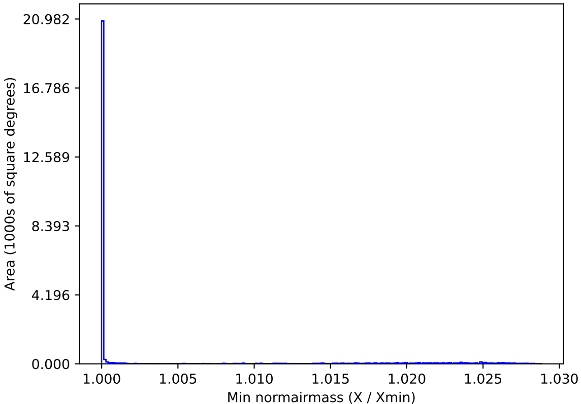
ddf_loaded_half_fl2_v3.4_10yrs All sky all bands: Min normairmass
