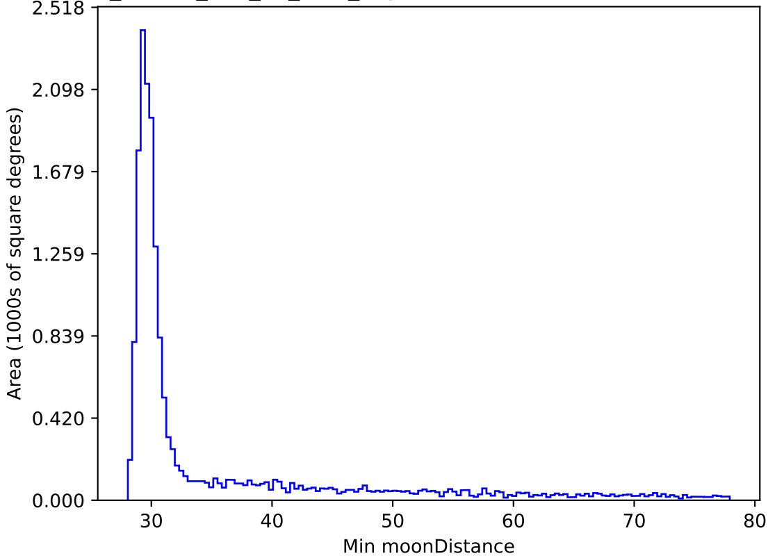
ddf_loaded_half_fl2_v3.4_10yrs WFD z band: Min moonDistance
