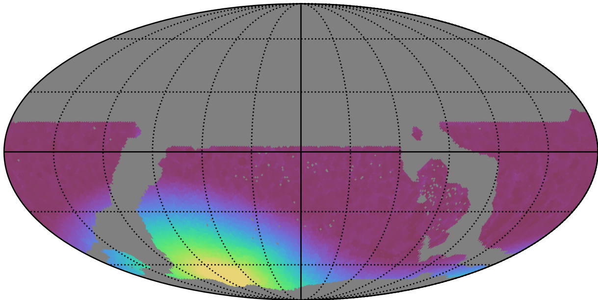
ddf_loaded_half_fl2_v3.4_10yrs WFD y band: Min moonDistance
