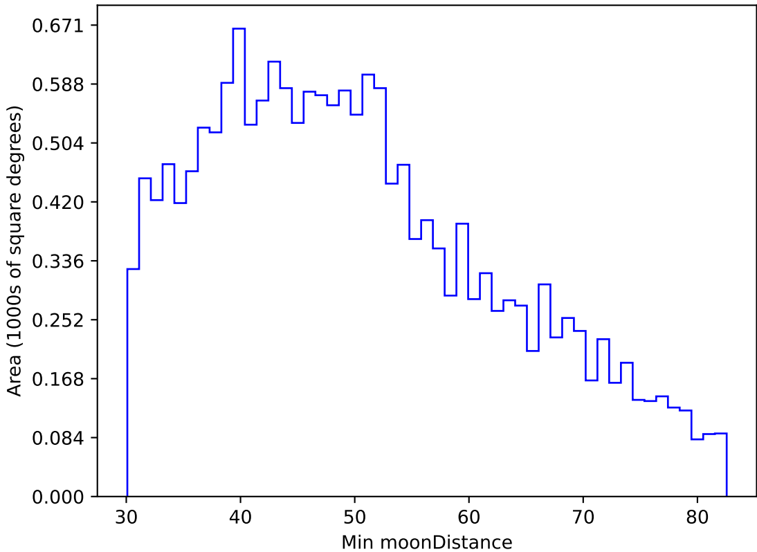
ddf_loaded_half_fl2_v3.4_10yrs WFD u band: Min moonDistance
