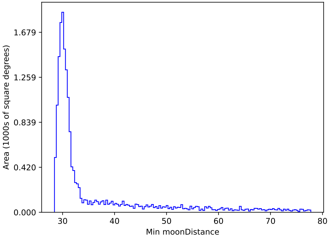
ddf_loaded_half_fl2_v3.4_10yrs WFD i band: Min moonDistance
