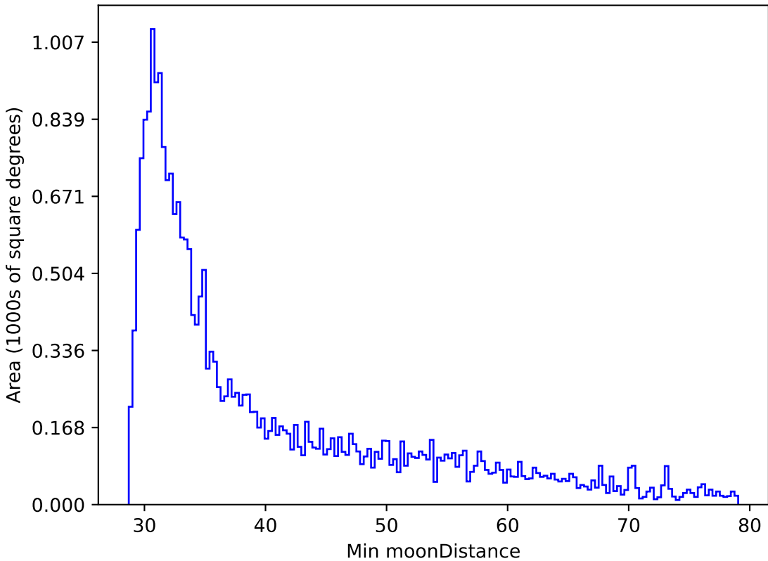
ddf_loaded_half_fl2_v3.4_10yrs All sky r band: Min moonDistance
