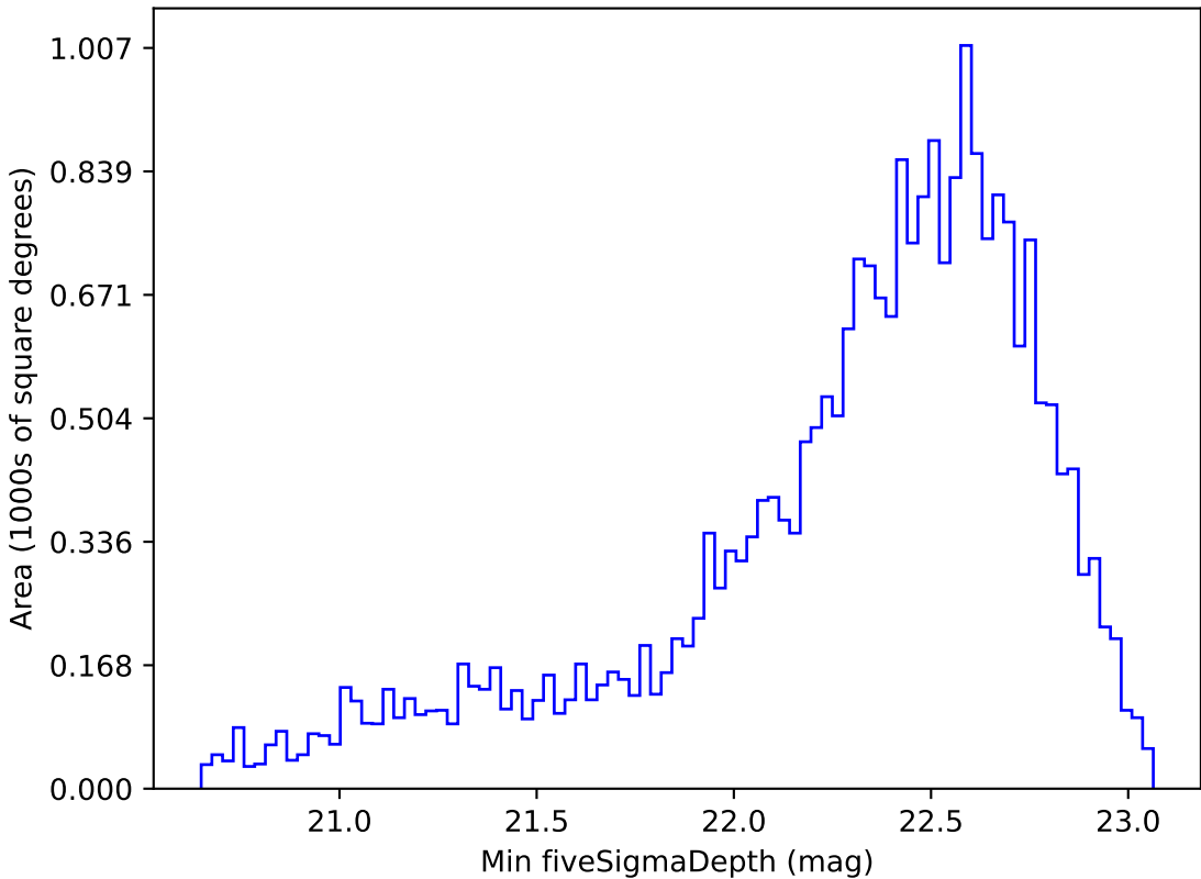
ddf_loaded_half_fl2_v3.4_10yrs Yr 1 z band: Min fiveSigmaDepth
