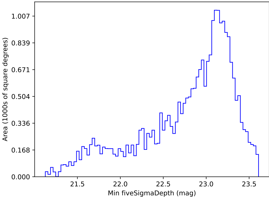
ddf_loaded_half_fl2_v3.4_10yrs Yr 1 i band: Min fiveSigmaDepth
