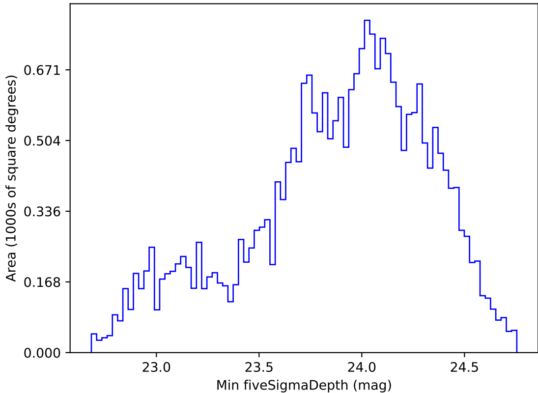
ddf_loaded_half_fl2_v3.4_10yrs Yr 1 g band: Min fiveSigmaDepth
