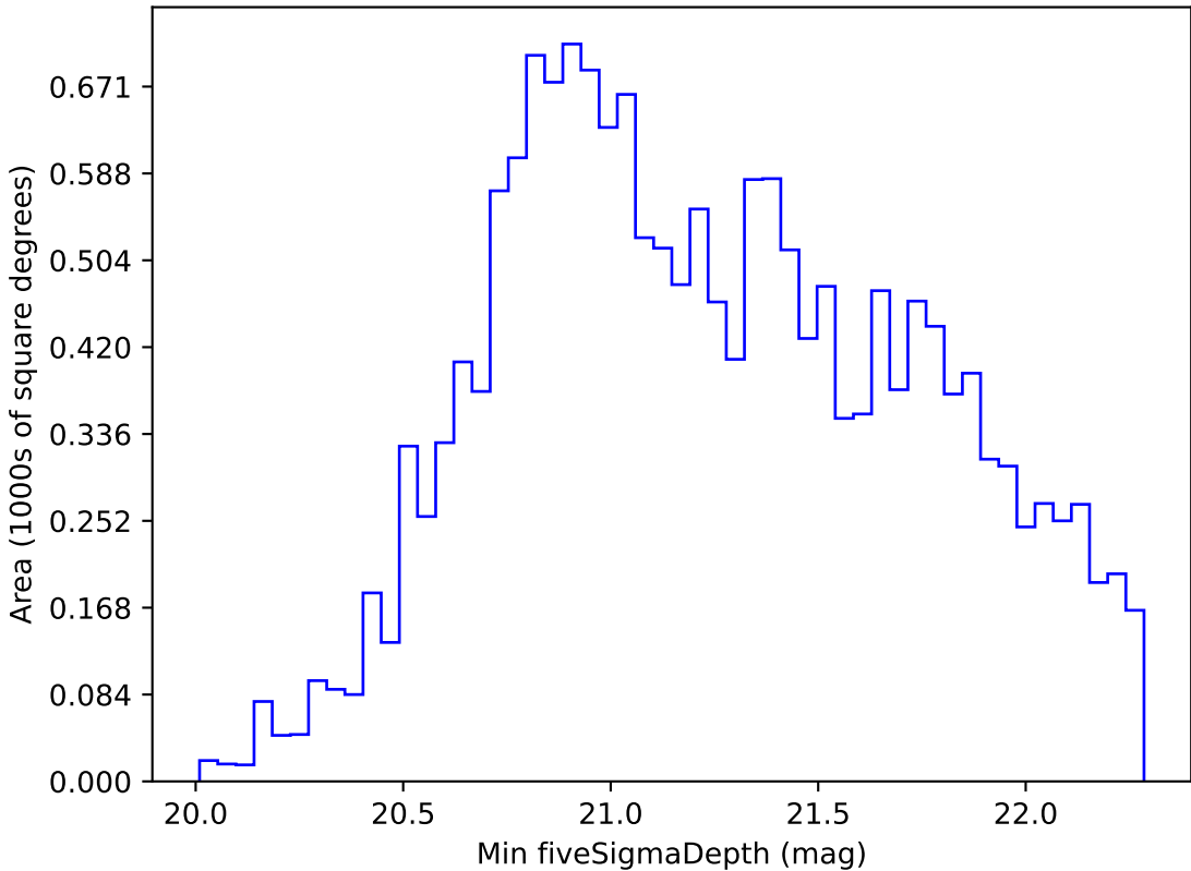
ddf_loaded_half_fl2_v3.4_10yrs WFD z band: Min fiveSigmaDepth
