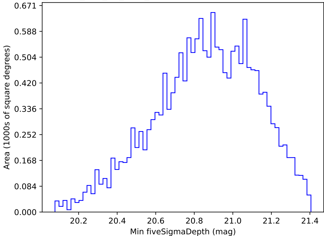
ddf_loaded_half_fl2_v3.4_10yrs WFD y band: Min fiveSigmaDepth
