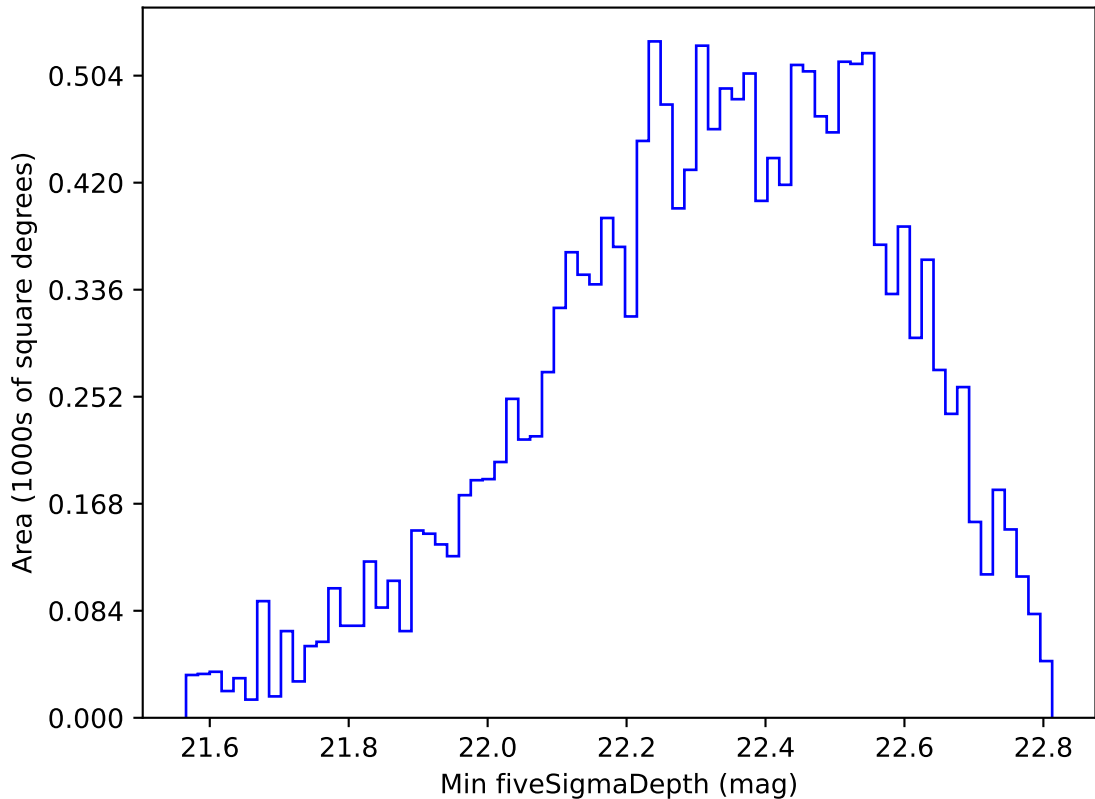
ddf_loaded_half_fl2_v3.4_10yrs WFD u band: Min fiveSigmaDepth
