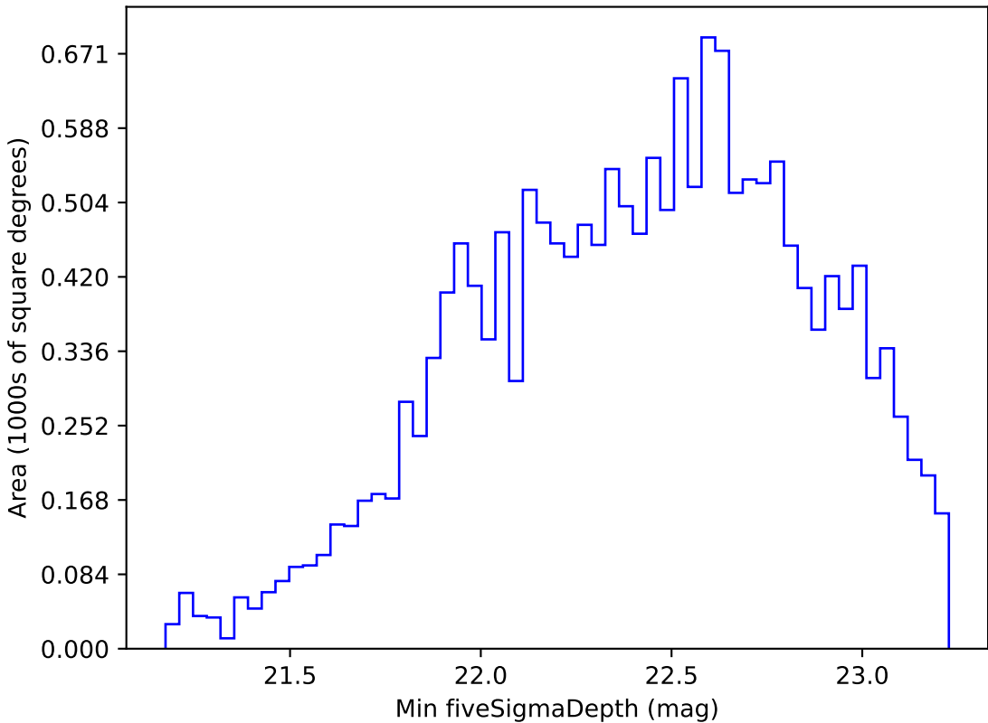
ddf_loaded_half_fl2_v3.4_10yrs WFD r band: Min fiveSigmaDepth
