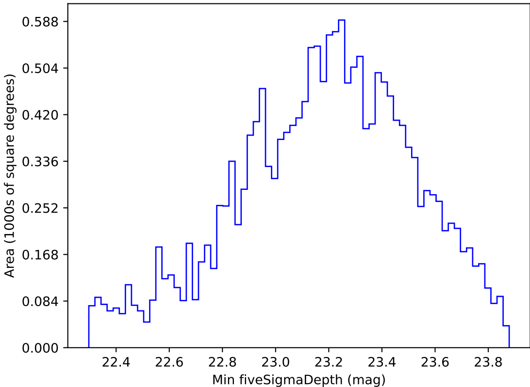
ddf_loaded_half_fl2_v3.4_10yrs WFD g band: Min fiveSigmaDepth
