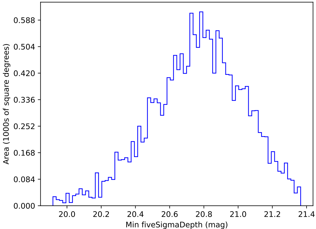
ddf_loaded_half_fl2_v3.4_10yrs WFD all bands: Min fiveSigmaDepth
