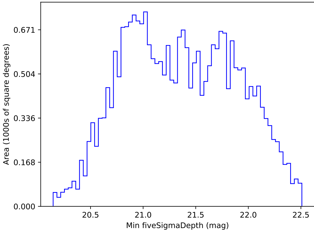
ddf_loaded_half_fl2_v3.4_10yrs All sky z band: Min fiveSigmaDepth
