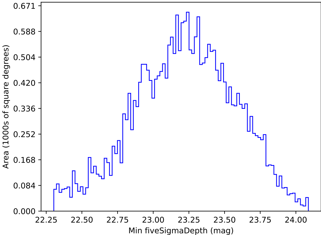
ddf_loaded_half_fl2_v3.4_10yrs All sky g band: Min fiveSigmaDepth
