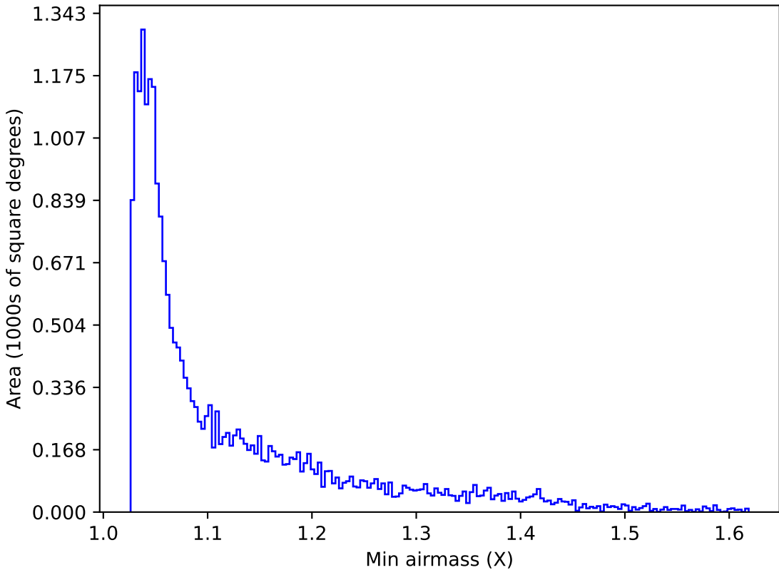
ddf_loaded_half_fl2_v3.4_10yrs Yr 1 y band: Min airmass
