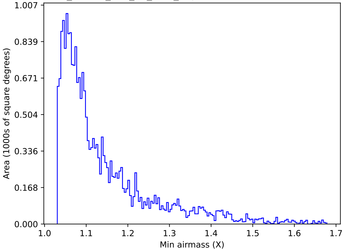
ddf_loaded_half_fl2_v3.4_10yrs Yr 1 u band: Min airmass
