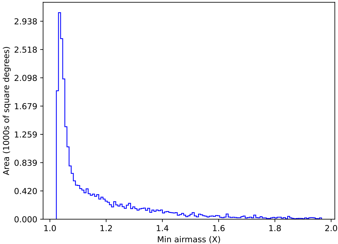
ddf_loaded_half_fl2_v3.4_10yrs Yr 1 r band: Min airmass
