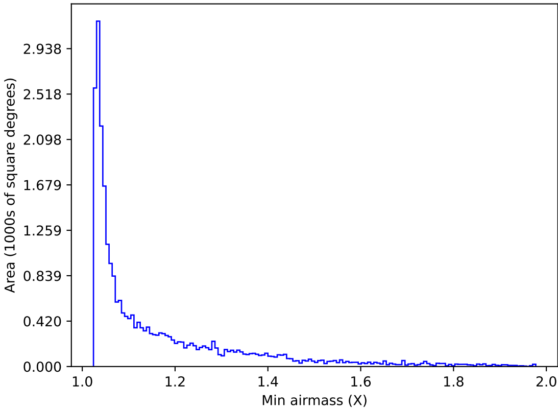
ddf_loaded_half_fl2_v3.4_10yrs Yr 1 i band: Min airmass
