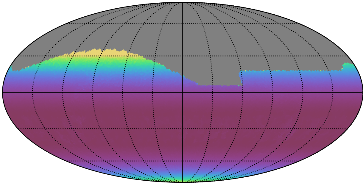
ddf_loaded_half_fl2_v3.4_10yrs Yr 1 all bands: Min airmass
