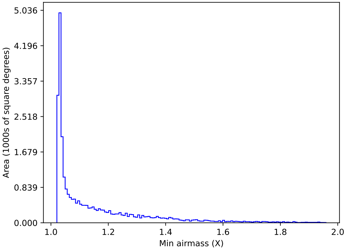
ddf_loaded_half_fl2_v3.4_10yrs Yr 1 all bands: Min airmass
