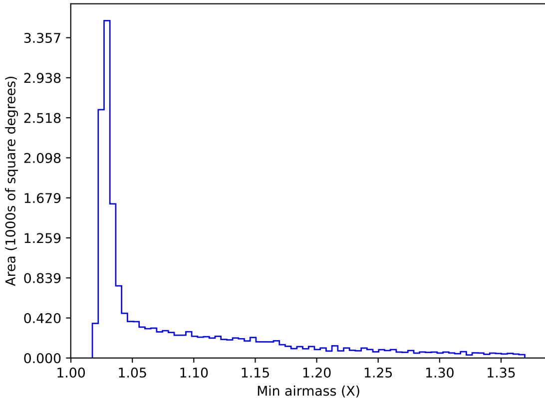
ddf_loaded_half_f12_v3.4_10yrs WFD z band: Min airmass
