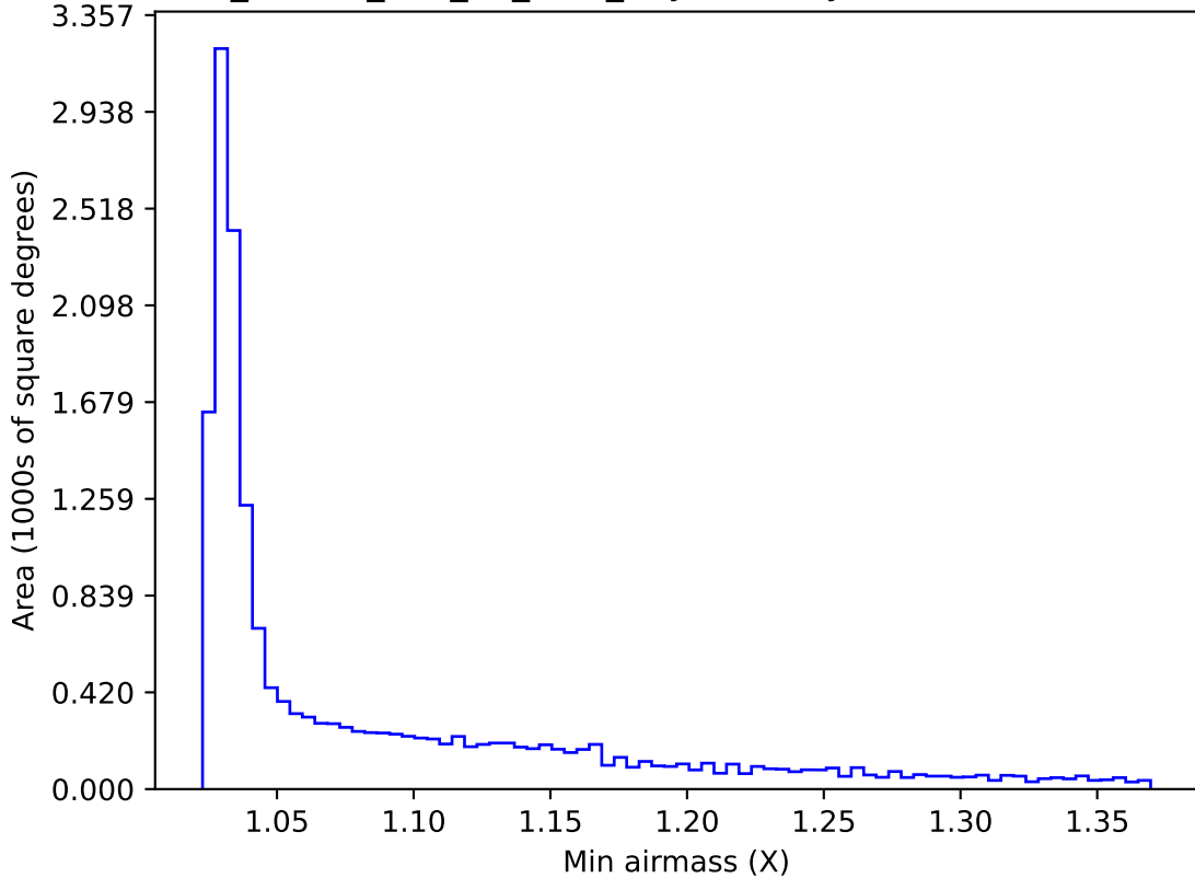
ddf_loaded_half_fi2_v3.4_10yrs WFD y band: Min airmass
