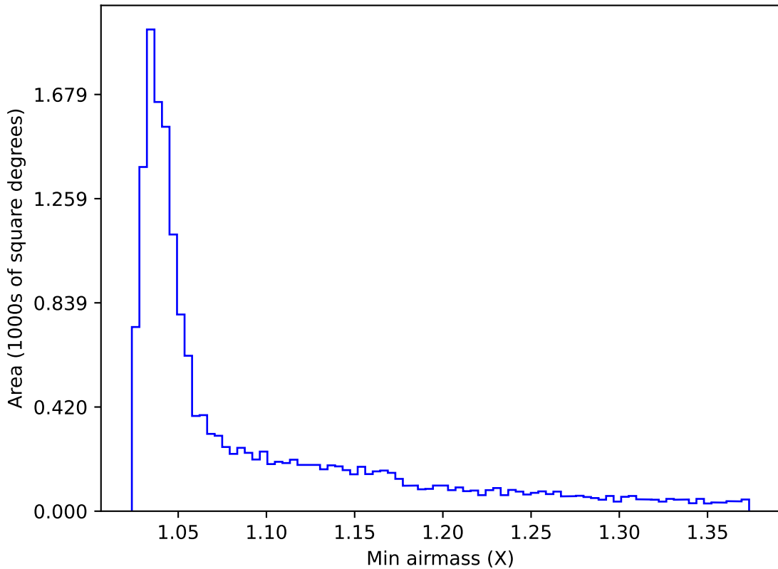
ddf_loaded_half_fl2_v3.4_10yrs WFD u band: Min airmass
