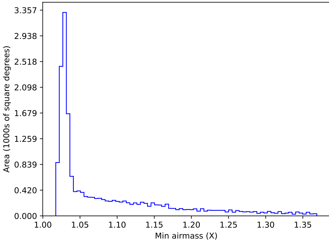
ddf_loaded_half_fl2_v3.4_10yrs WFD i band: Min airmass
