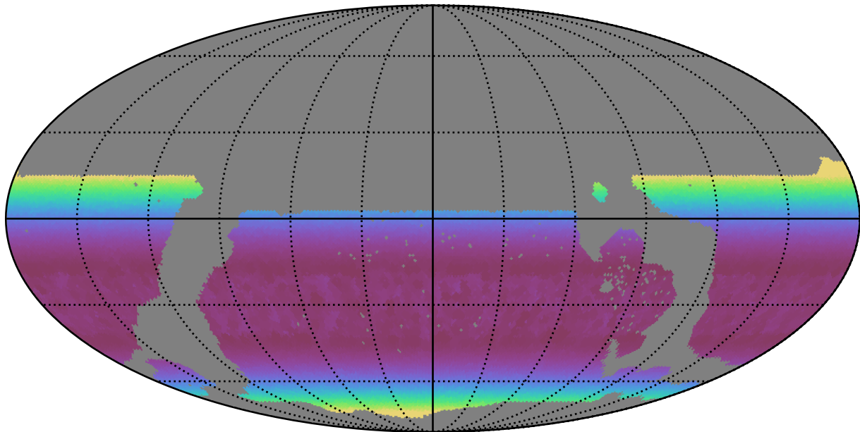
ddf_loaded_half_fl2_v3.4_10yrs WFD g band: Min airmass
