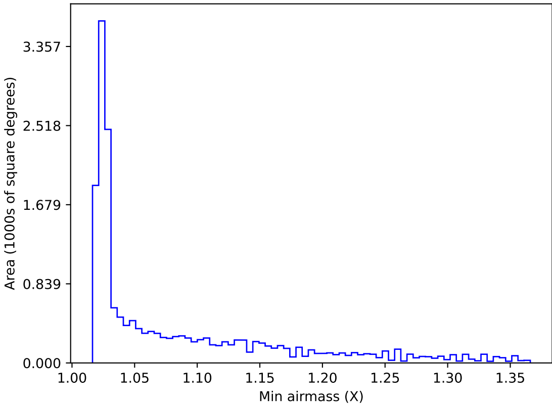
ddf_loaded_half_fl2_v3.4_10yrs WFD all bands: Min airmass
