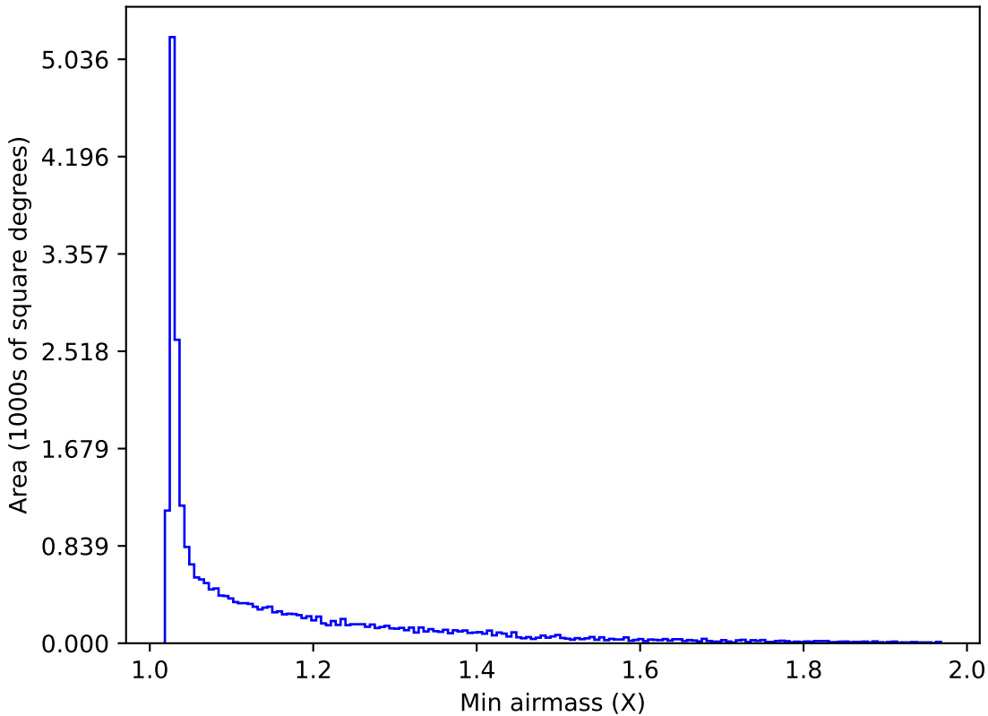
ddf_loaded_half_fl2_v3.4_10yrs All sky z band: Min airmass
