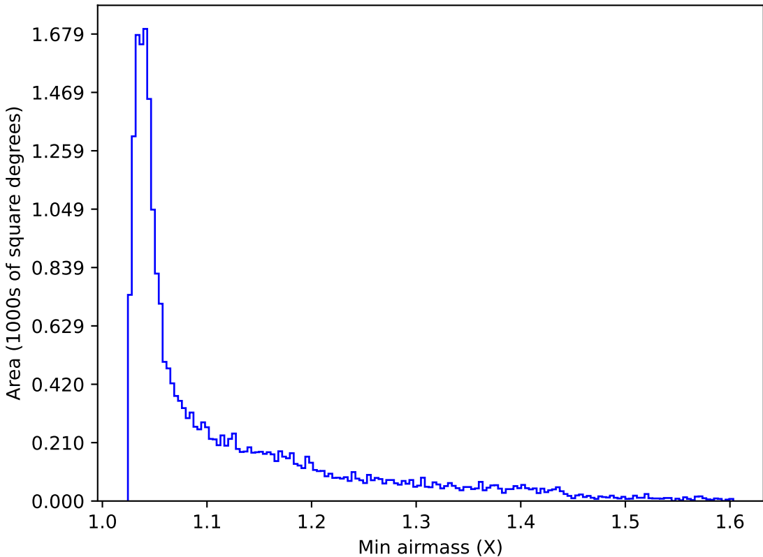
ddf_loaded_half_fl2_v3.4_10yrs All sky u band: Min airmass
