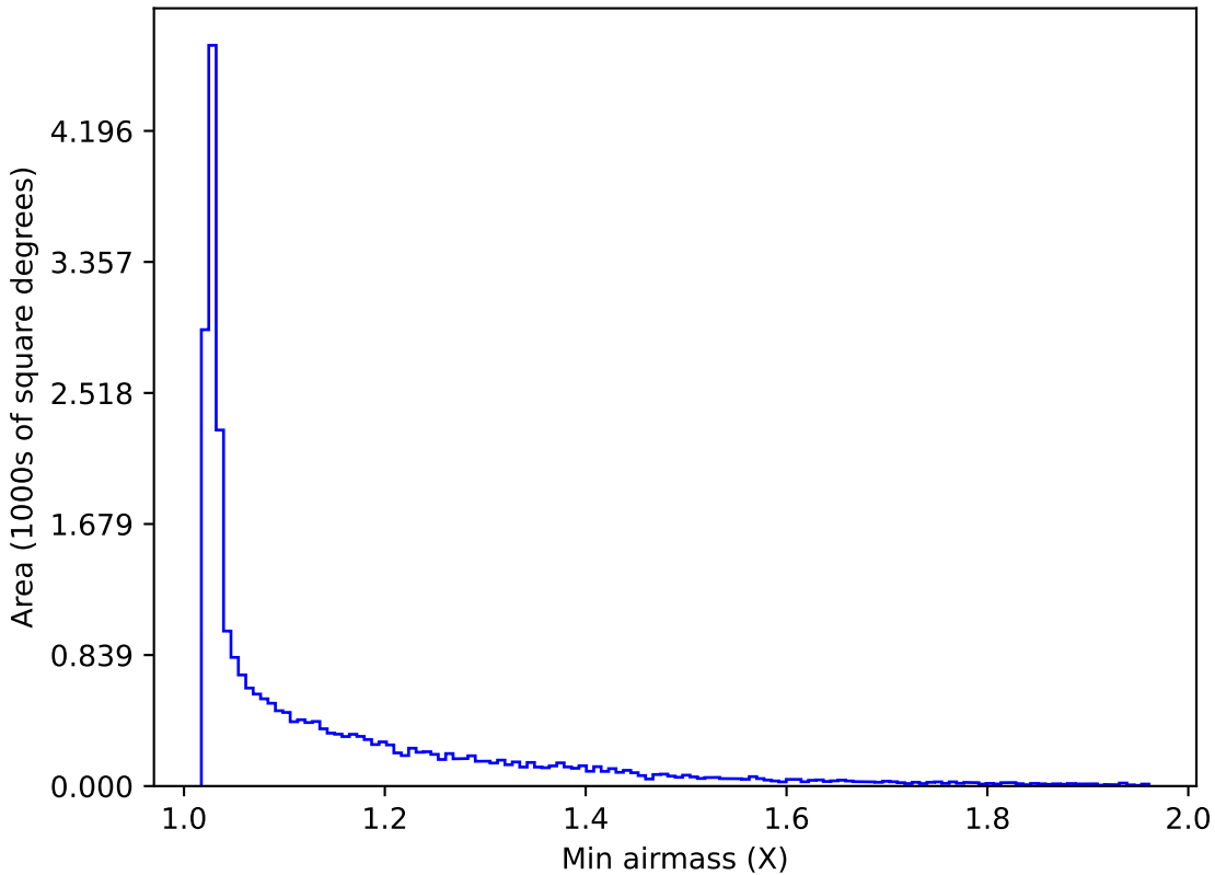
ddf_loaded_half_fl2_v3.4_10yrs All sky r band: Min airmass
