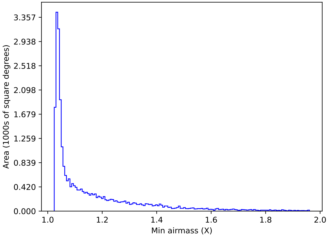
ddf_loaded_half_fl2_v3.4_10yrs All sky g band: Min airmass
