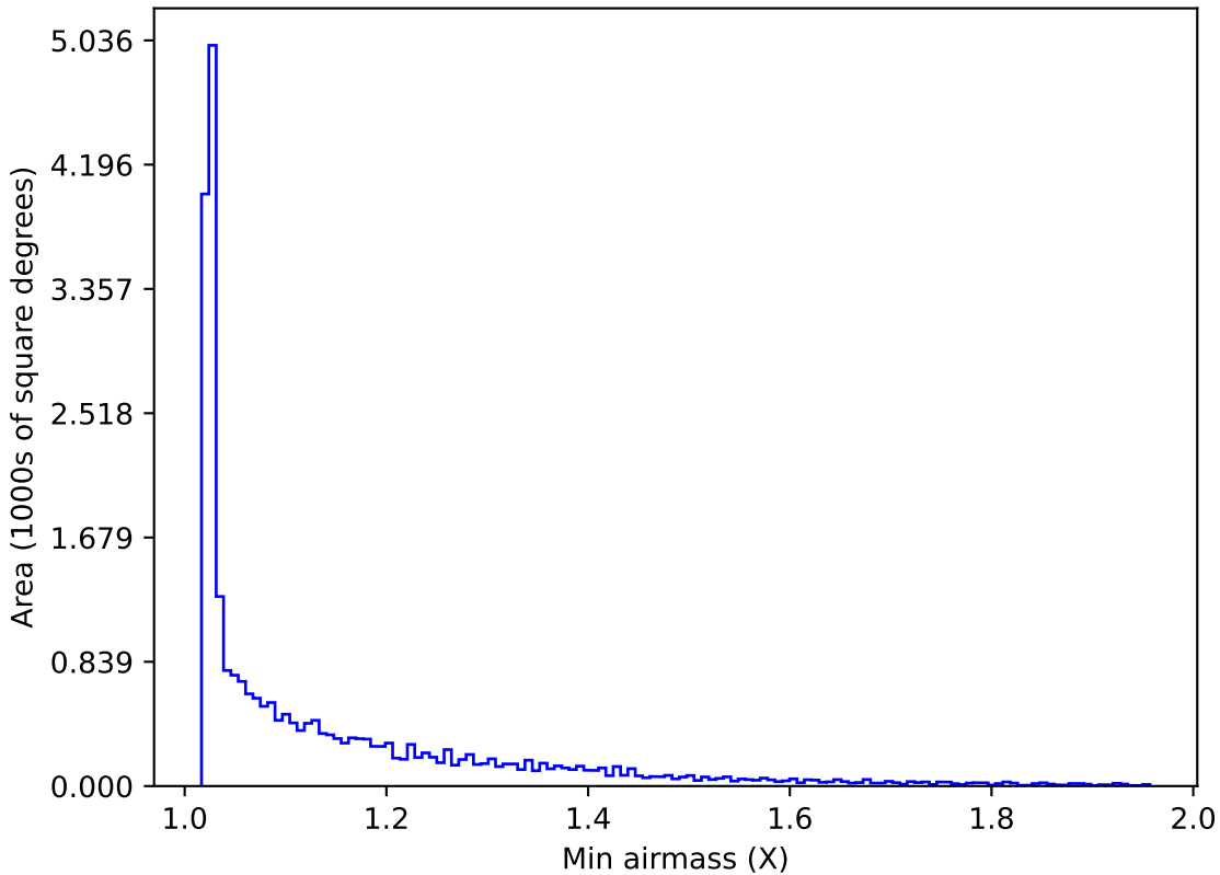
ddf_loaded_half_fl2_v3.4_10yrs All sky all bands: Min airmass
