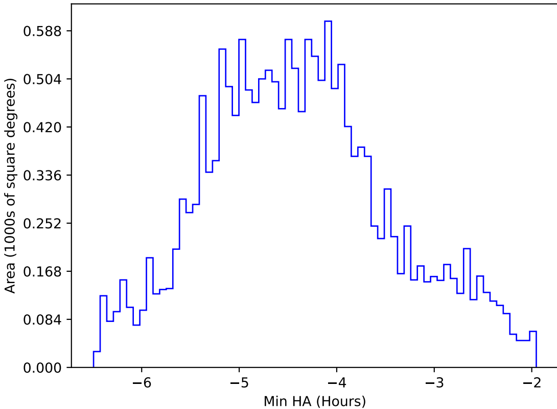
ddf_loaded_half_fl2_v3.4_10yrs WFD z band: Min HA
