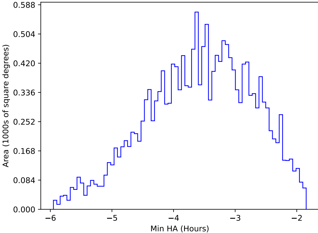
ddf_loaded_half_fl2_v3.4_10yrs WFD y band: Min HA
