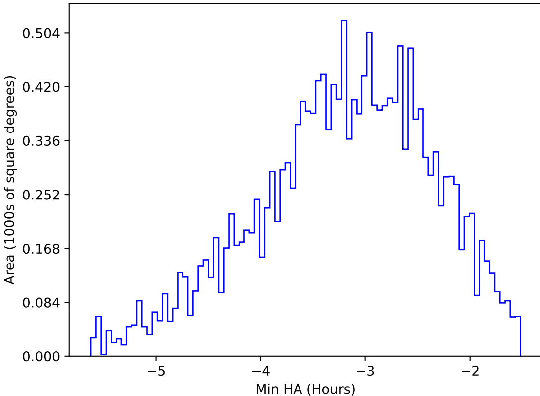
ddf_loaded_half_fl2_v3.4_10yrs WFD u band: Min HA
