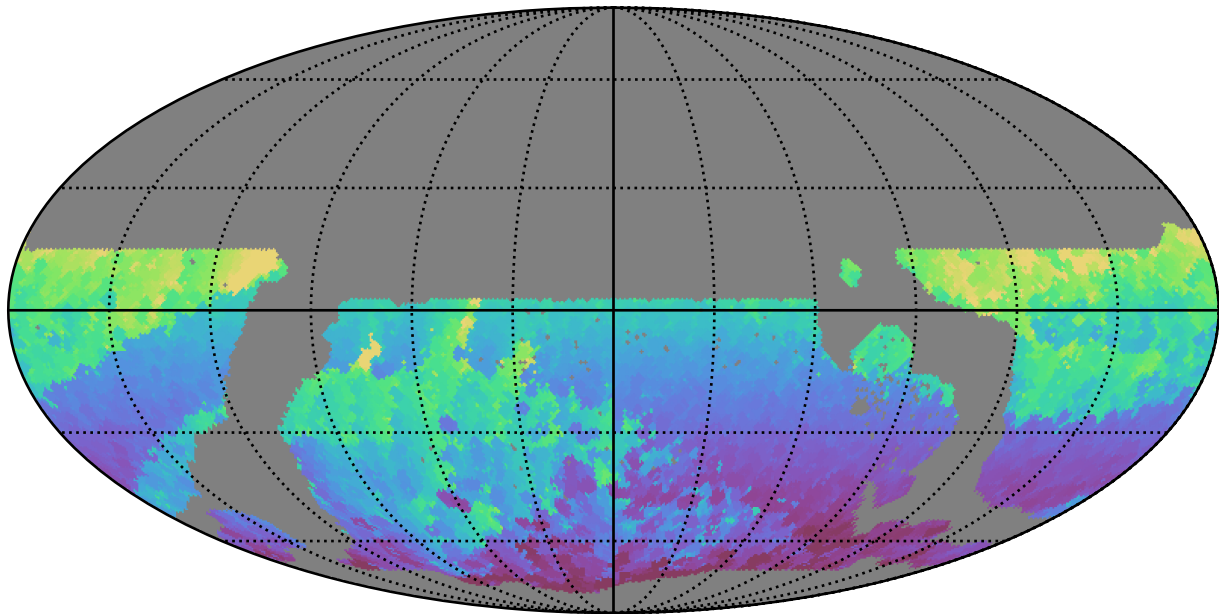
ddf_loaded_half_fl2_v3.4_10yrs WFD r band: Min HA
