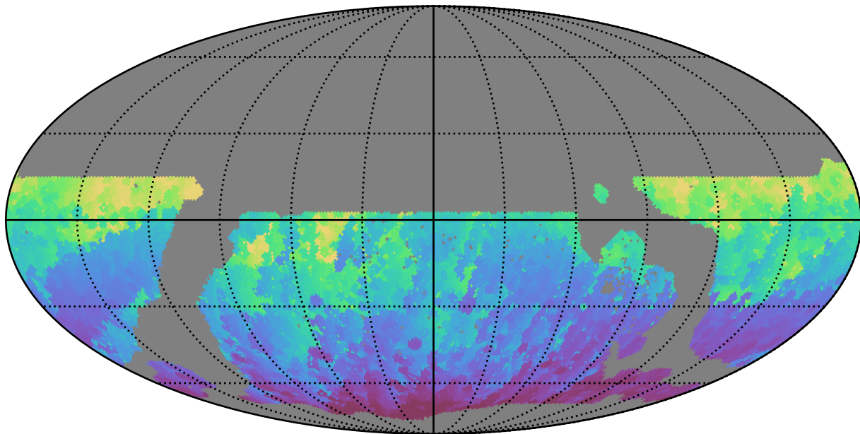
ddf_loaded_half_fl2_v3.4_10yrs WFD i band: Min HA
