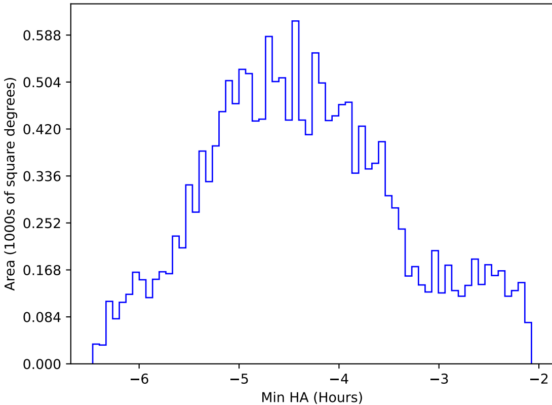
ddf_loaded_half_fl2_v3.4_10yrs WFD i band: Min HA
